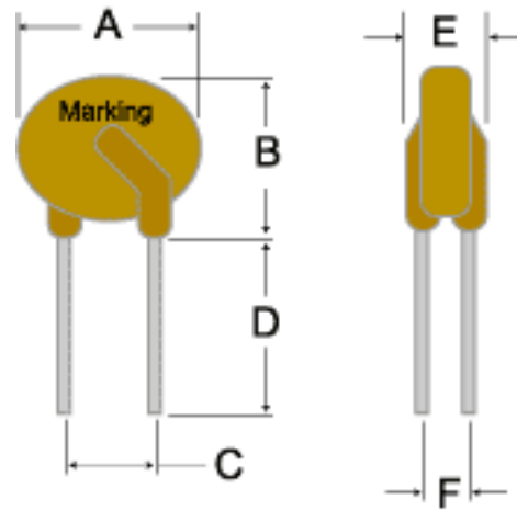
Figure 2 RX110-60 ~ RX375-60 Lead Size : 20AWG, Ø 0.81 mm Diameter
