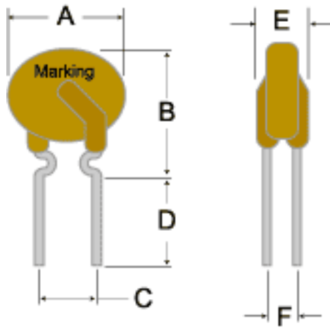
Figure 1 RX005-60 ~ RX090-60 Lead Size :24AWG, Ø 0.51 mm Diameter
