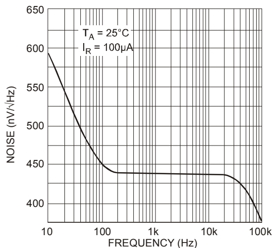
Noise Voltage vs. Frequency LM4040-30
