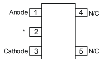
SC70-5**
