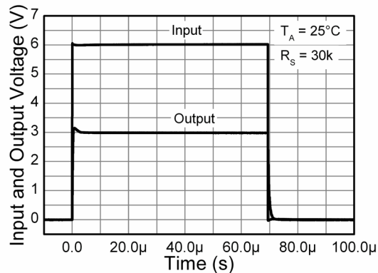
Long Pulse Response LM4040-30
