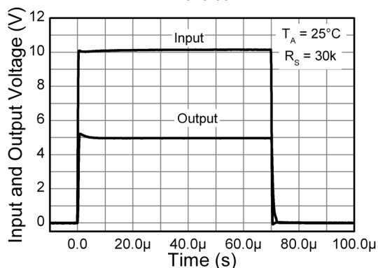
Long Pulse Response LM4040-50
