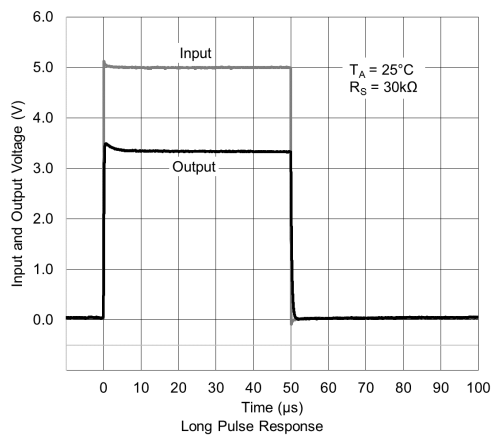
Long Pulse Response LM4040-33
