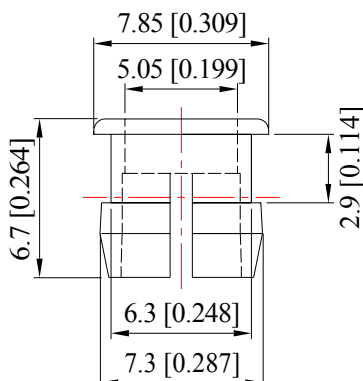
Panel Mount Clip
