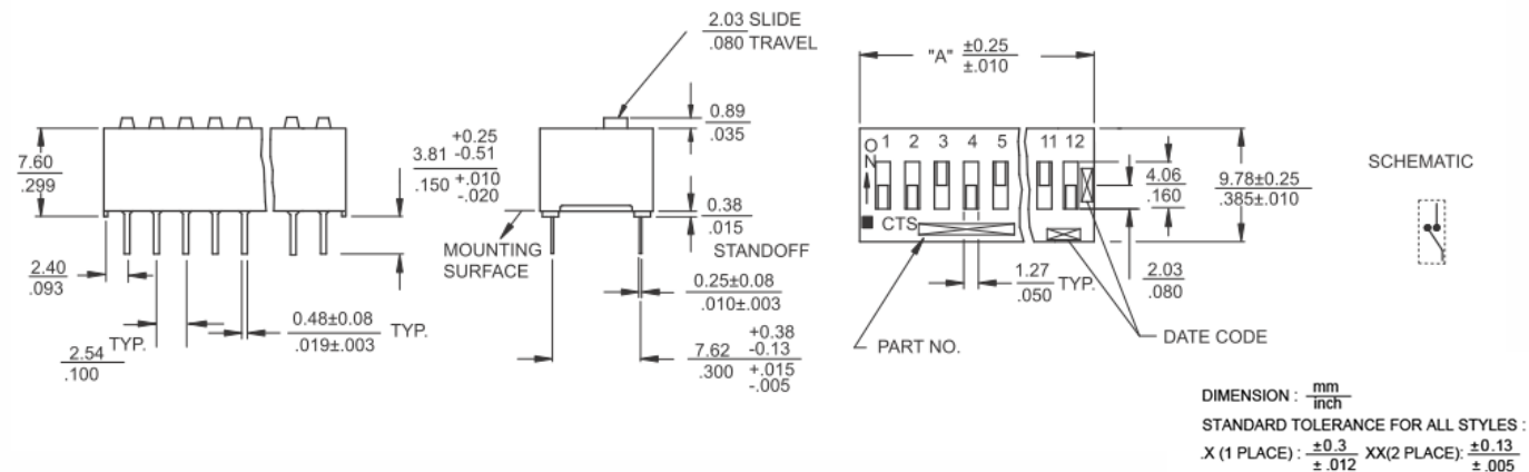
Figure 1 - SPST
