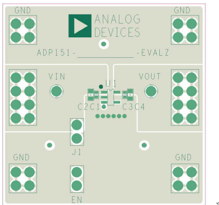
Figure 60. Example TSOT PCB Layout
