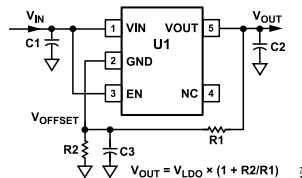
Figure 33. Adjustable LDO Using the ADP151
