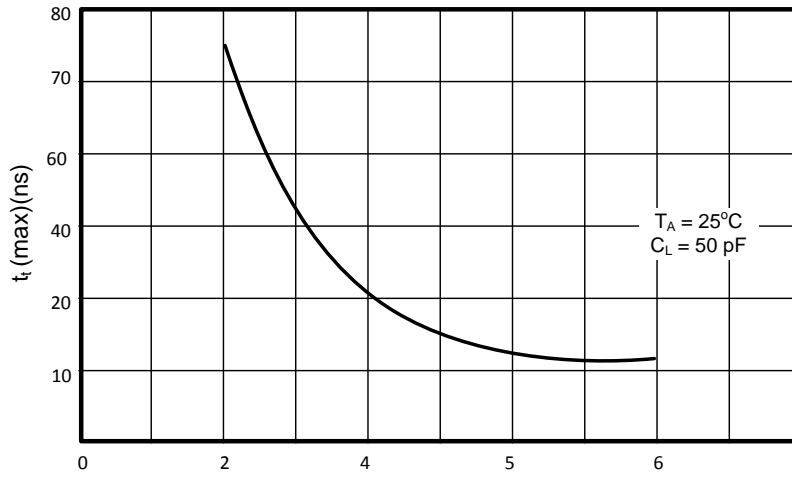
Figure 1. t_t vs V_{CC}
