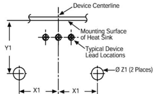
Mounting Details:
