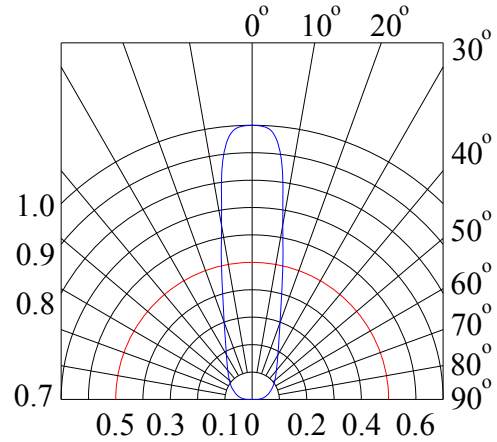
Radiation Diagram
