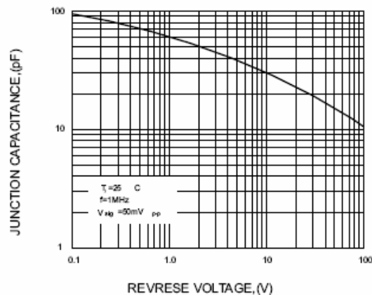
FIG.5-TYPICAL JUNCTION CAPACITANCE
