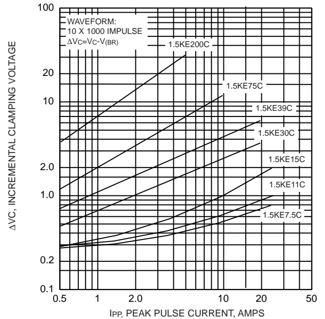
FIG. 10 - INCREMENTAL CLAMPING VOLTAGE CURVE BI-DIRECTIONAL
